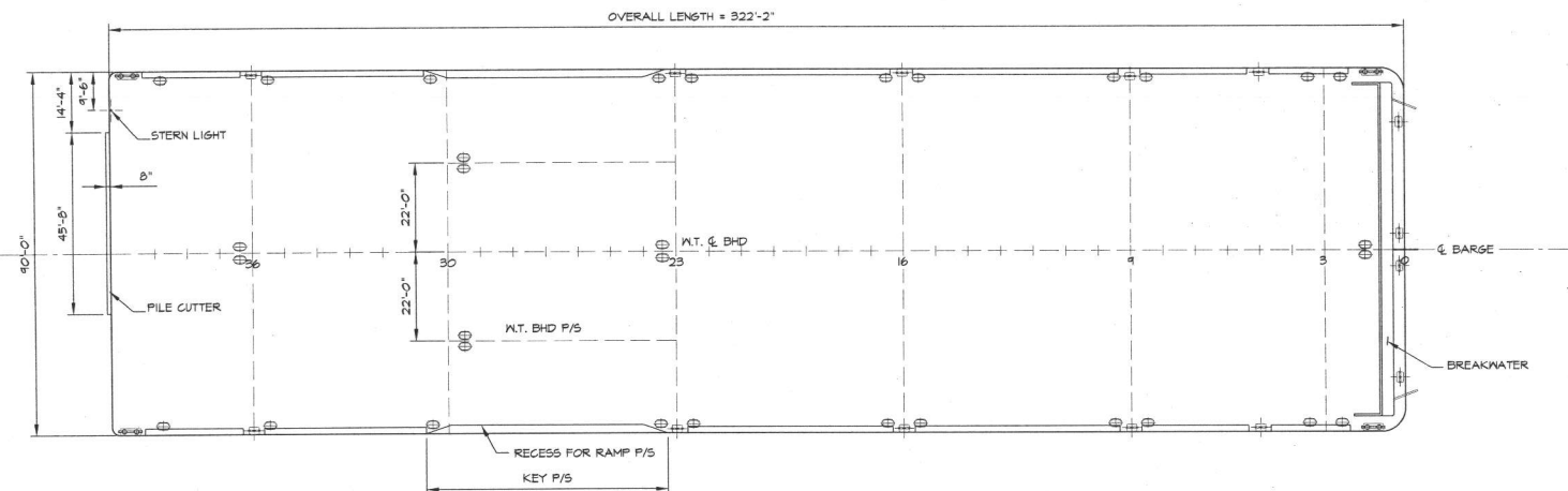
MAIN DECK ARRANGEMENT
