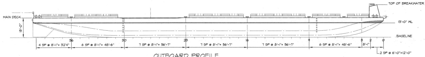
OUTBOARD PROFILE
