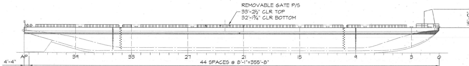
OUTBOARD PROFILE
