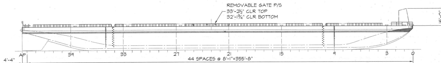
OUTBOARD PROFILE
