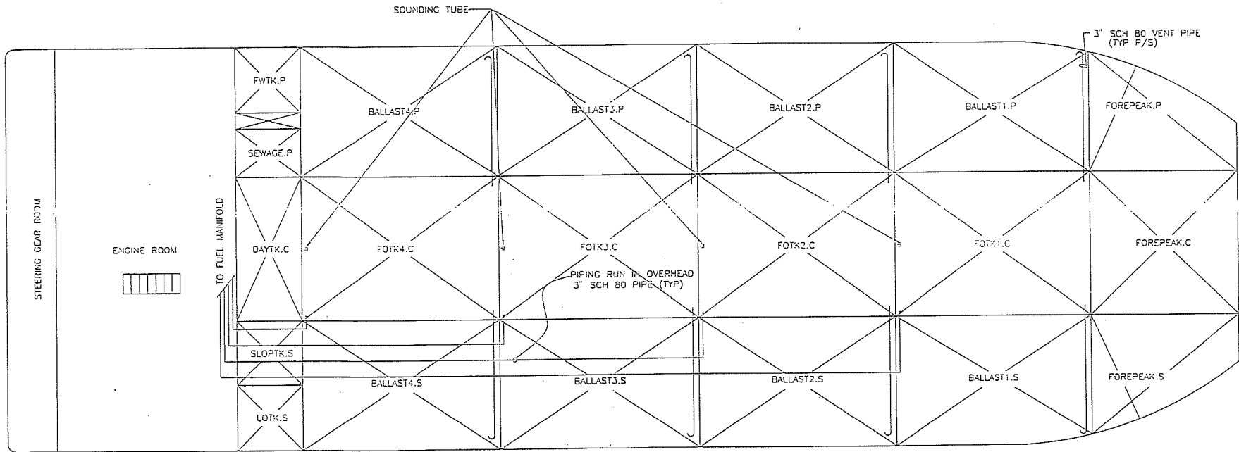
TANK PLAN
