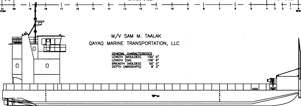
OUTBOARD PROFILE
