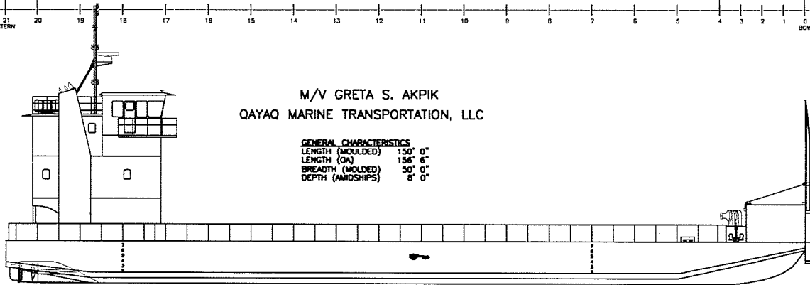
OUTBOARD PROFILE
