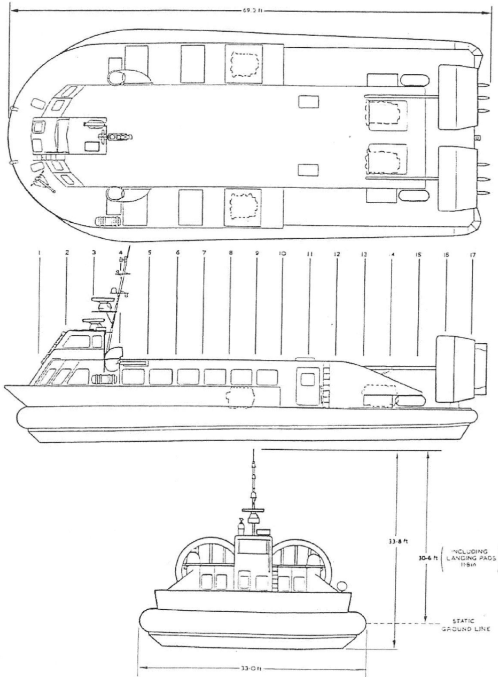
FIGURE 1 - GENERAL ARRANGEMENT
