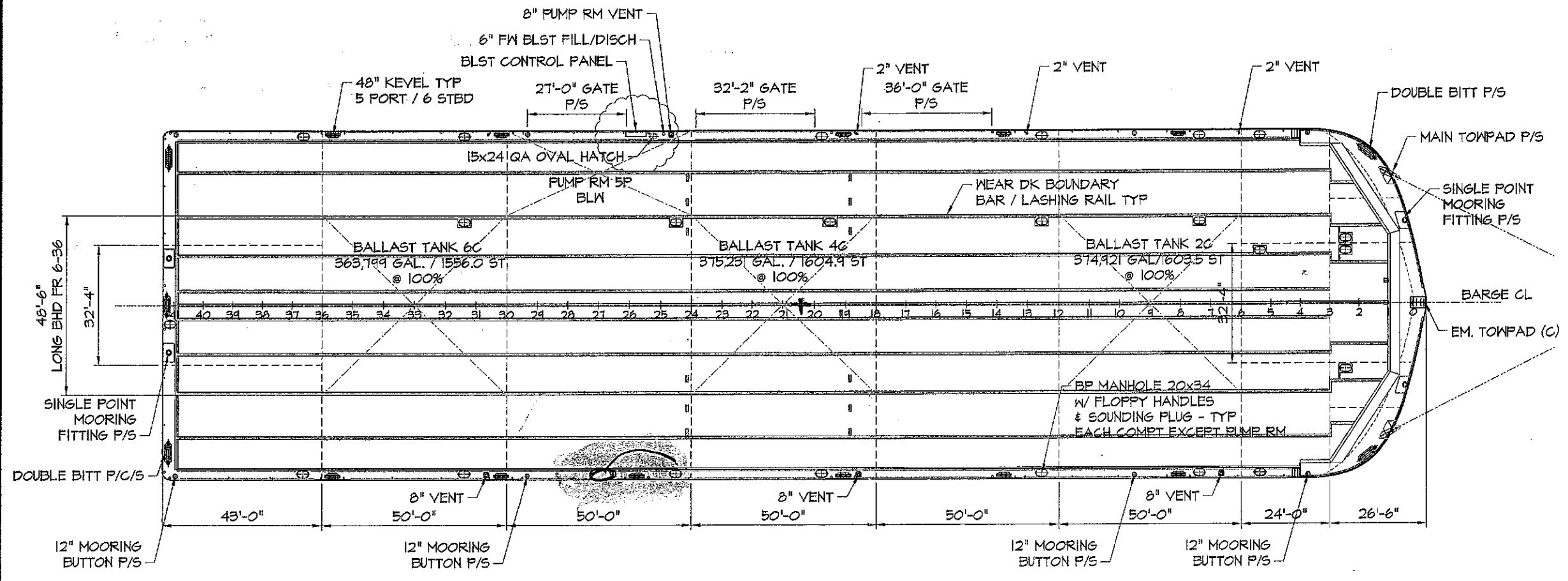
MAIN DECK PLAN SCALE: 1/32" = 1'-0"
