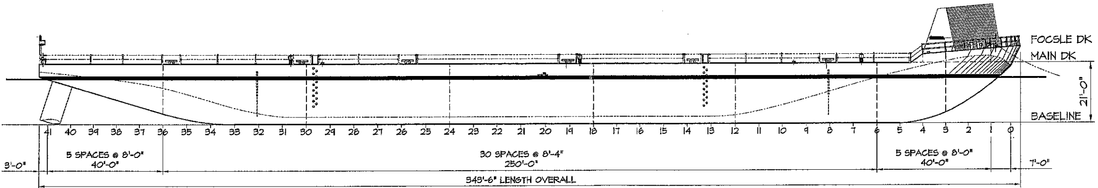
OUTBOARD PROFILE SCALE: 1/32" = 1'-0"
